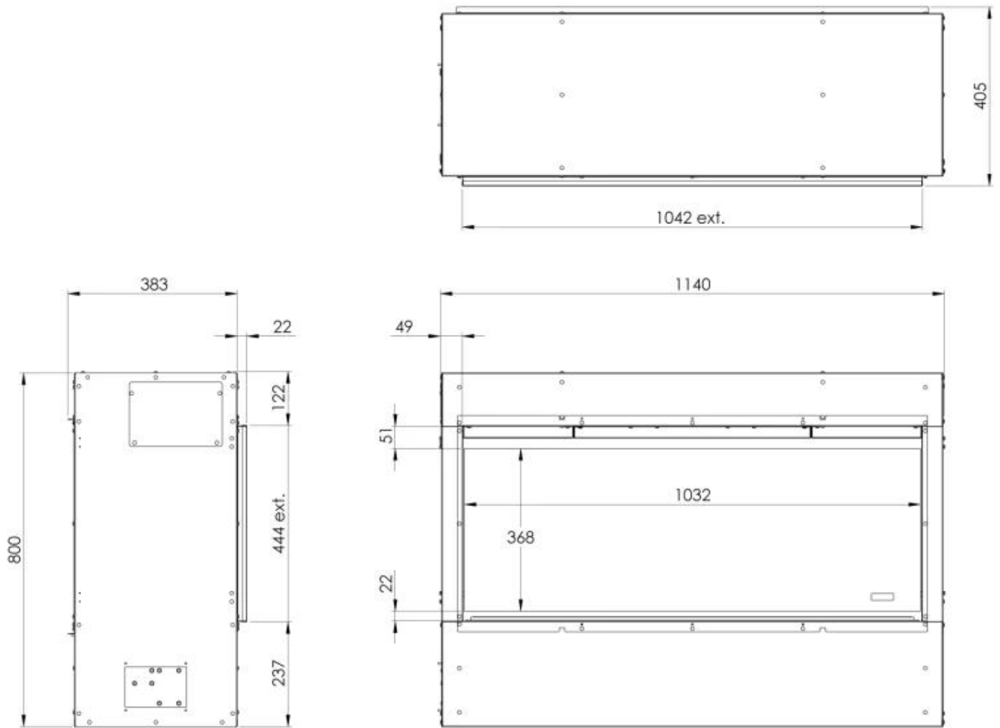
Dimensional drawing e-BoX 1000/450 I
